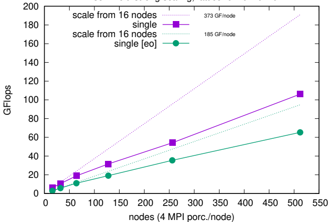
Wilson mult: strong scaling, lattice=64x64x64x64
