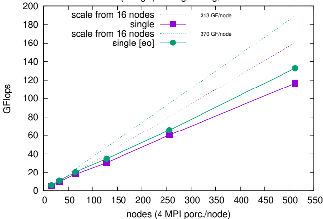
Domainwall mult (DdagD): strong scaling, lattice=64x64x64x64
